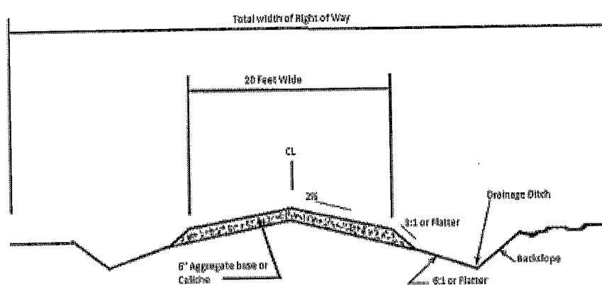
Torrance County Typical Road Section
